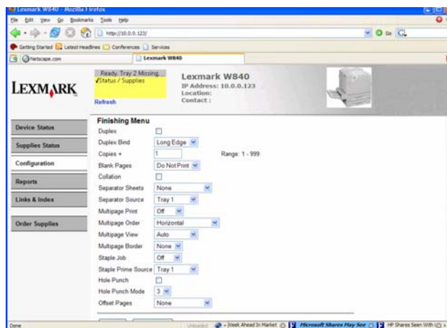
The Web interface lets you select finishing options, like duplexing and hole punching.
