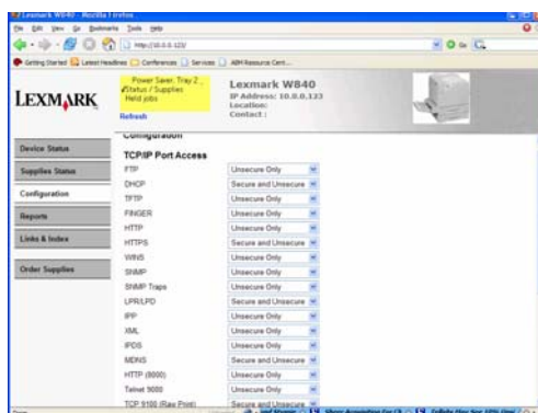
With Lexmark printers, IPsec can be enabled on a port basis.
