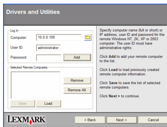
The Lexmark W840 lets you install the driver onto multiple workstations.
